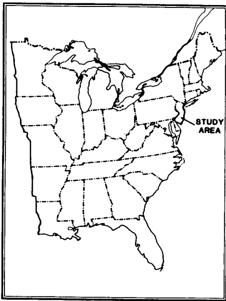
FIGURE 3-1 THE SOUTH CENTRAL NEW JERSEY STUDY AREA
